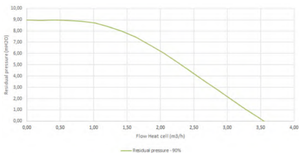
Pump head diagram, boiler type 100
