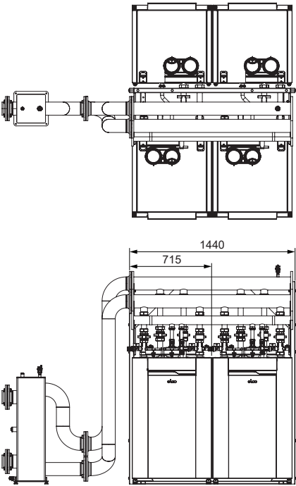
TRIGON L PLUS 4 boilers floor standing back-to-back
