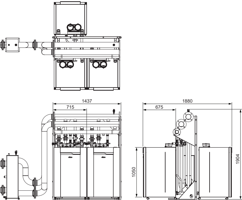
TRIGON L PLUS 6 boilers floor standing back-to-back
