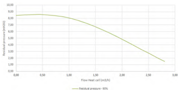
Pump head diagram, boiler type 60 – 70
