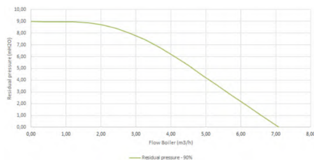
Pump head diagram, boiler type 170 – 200
