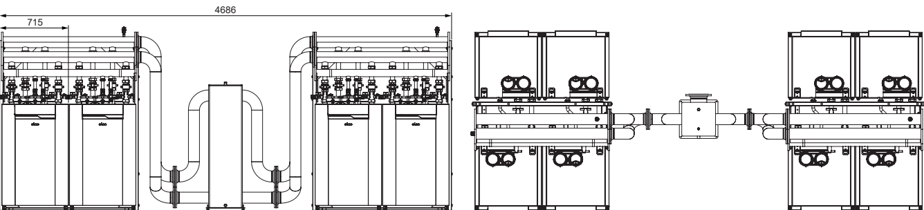
TRIGON L PLUS 8 boilers floor standing back-to-back
