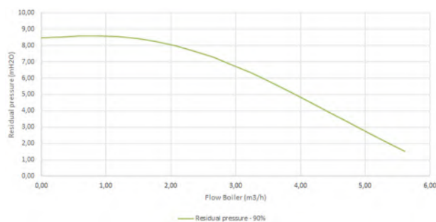
Pump head diagram, boiler type 120 – 140
