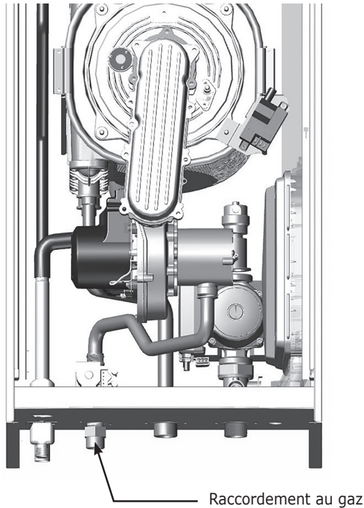
FIGURE 7-1 Raccordement au gaz
