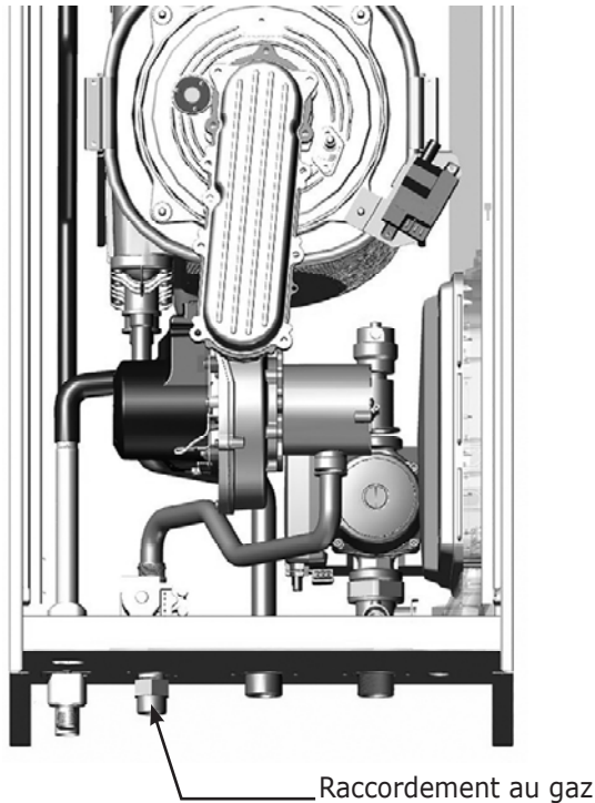
FIGURE 7-1 Raccordement au gaz
