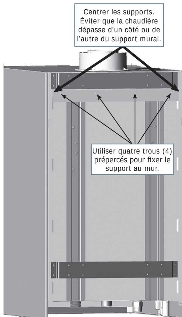
Figure 4-3 Support mural (inclus)
